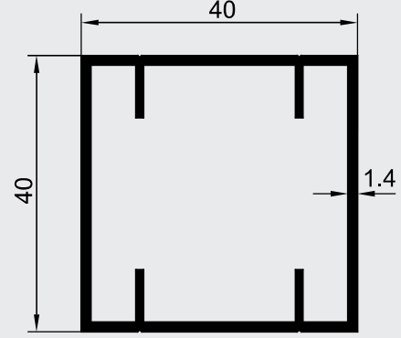
GLS-4013 KG:0.678
